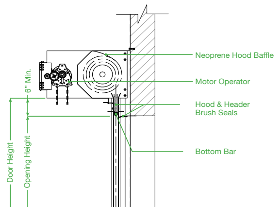
HEAD DETAIL SECTION
