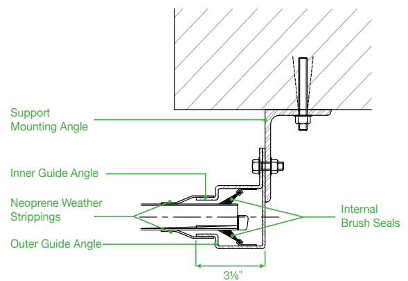
FACE OF WALL MOUNT GUIDE DETAILS
